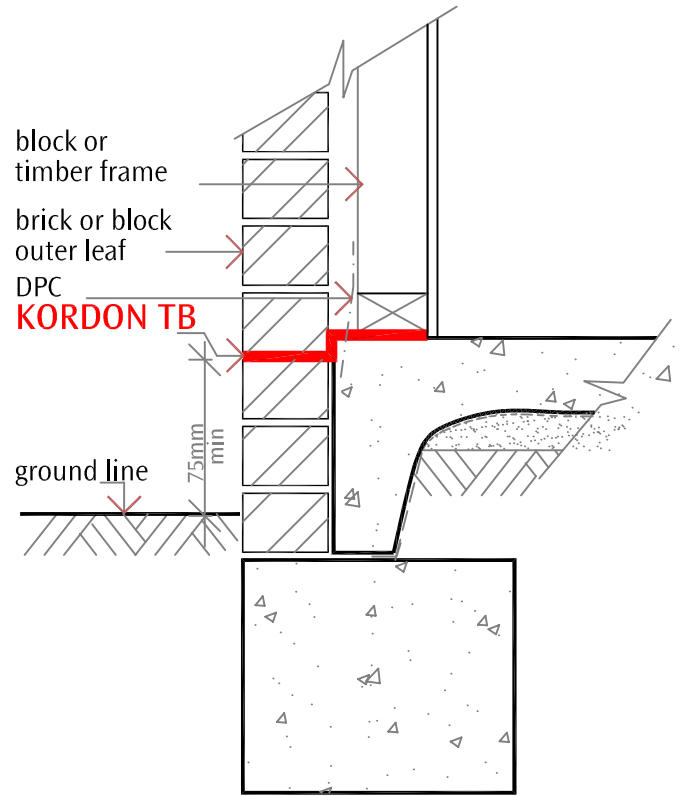
section detail 4
